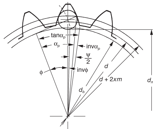
Fig. 10-10 Between Pin Dimension of Internal Gears
