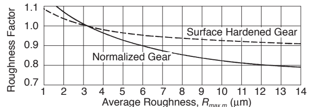
Fig. 17-4 Surface Roughness Factor, Z_R
