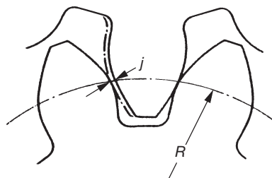
Figure 14-1 Backlash, j , Between Two Gears
