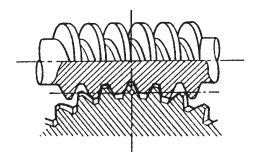
Fig. 2-17 Worm Gear
