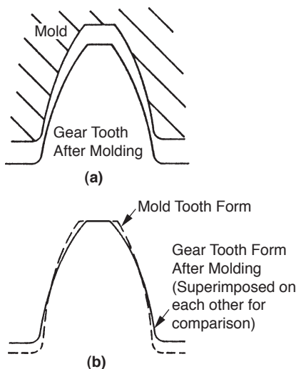
Fig. 18-8 Change of Tooth Profile
