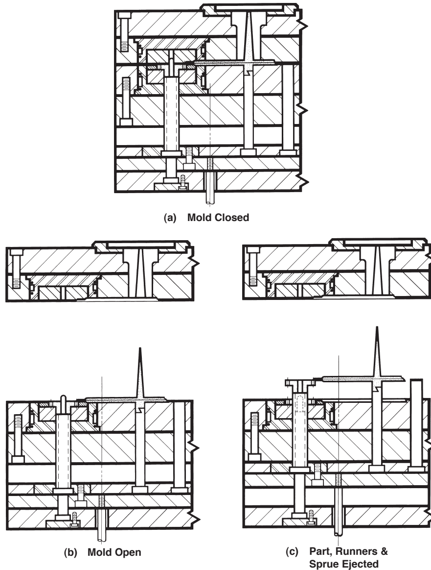
Fig. 18-15 Two-Plate Mold
