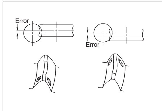
Fig. 19-8 Poor Contact Due to Mounting Distance Error
