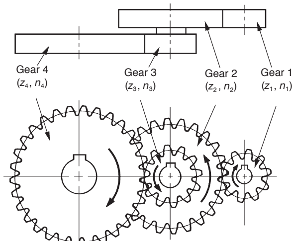
Fig. 13-2 Two-Stage Gear Train
